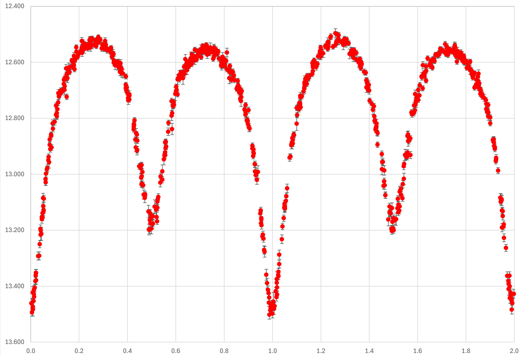
ASAS J221652+2229.6 R-Filter Source_AMag_T1
